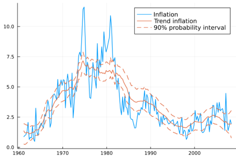
Figure 6: Inflation and trend inflation - Piecewise linear model.
