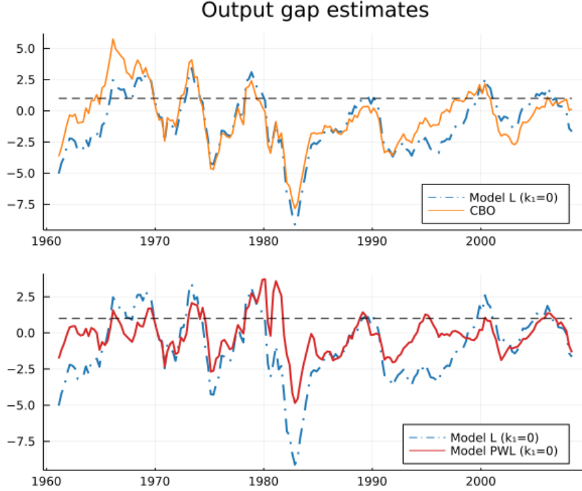
Figure 8: Comparison between short-run output gap estimates.
