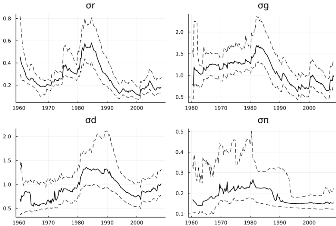
Figure 10: Stochastic volatility of the structural shocks
