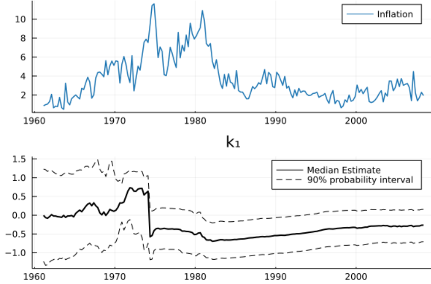
Figure 2: Online inference of the slope k_1 - Linear model.
