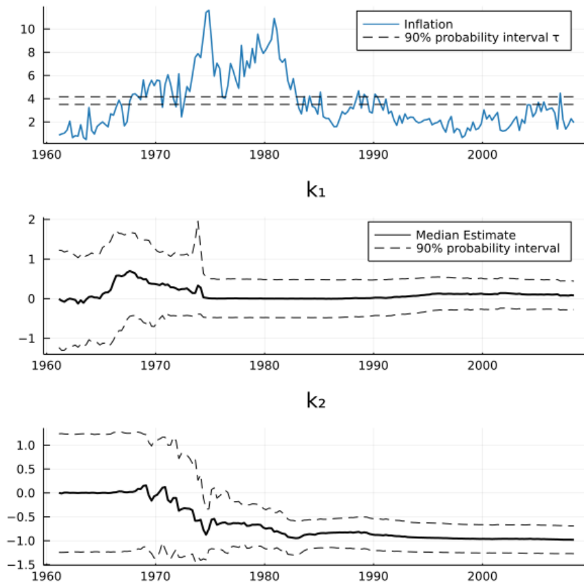
Figure 4: Online inference of the slopes k_1 and k_2 - Piecewise linear model.
