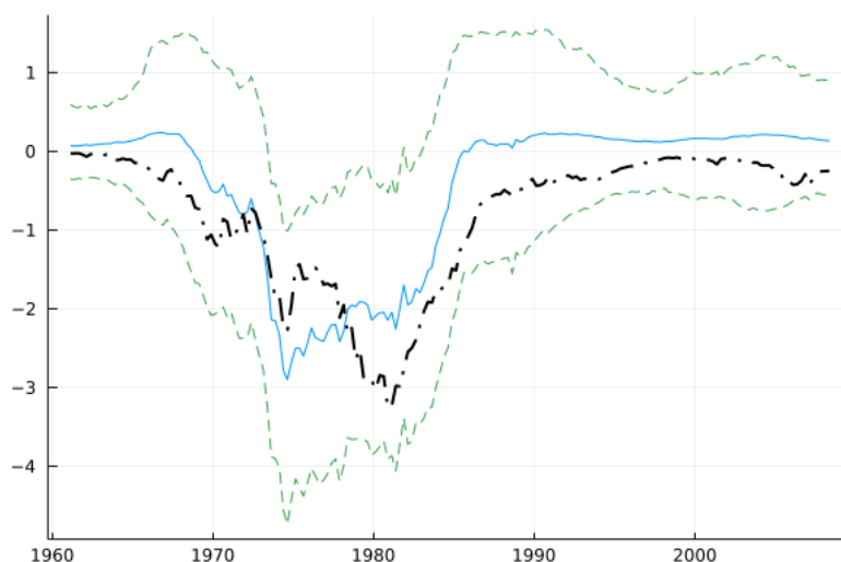
Figure 12: Comparison between long-run output gap estimates: VAR (blue) and GNK (black).
