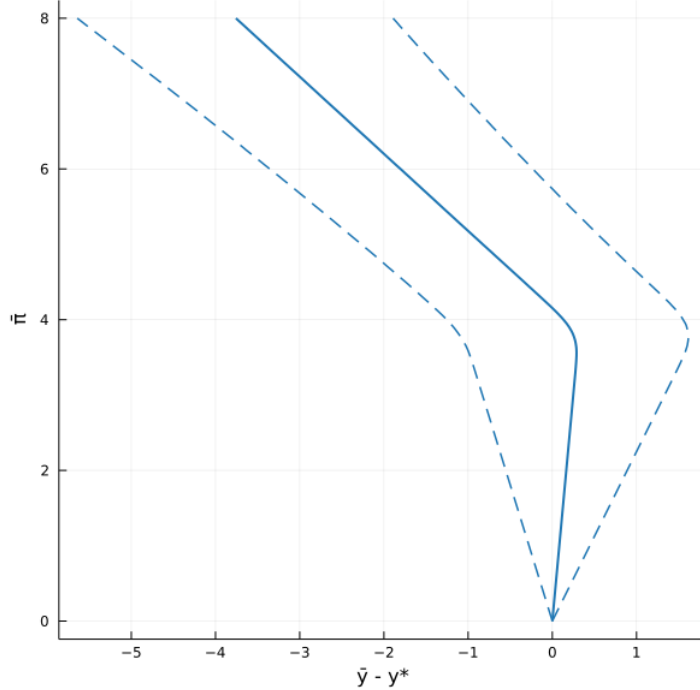
Figure 5: Long-run Phillips curve estimated through the piecewise linear model: median (continuous line) and 90% probability interval (dashed lines).
