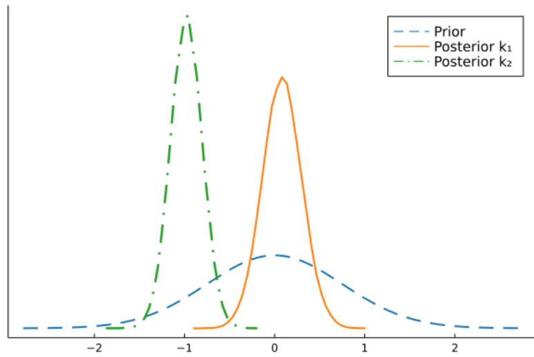
Figure 3: Estimates of the slopes of the long-run Phillips curve - Piecewise linear model.
