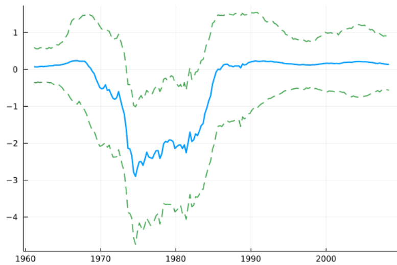
Figure 7: Long-run output gap estimated through the piecewise linear model.
