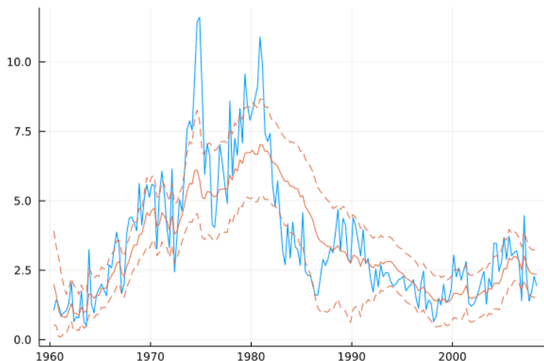
Figure 9: Inflation and trend inflation - GNK model.
