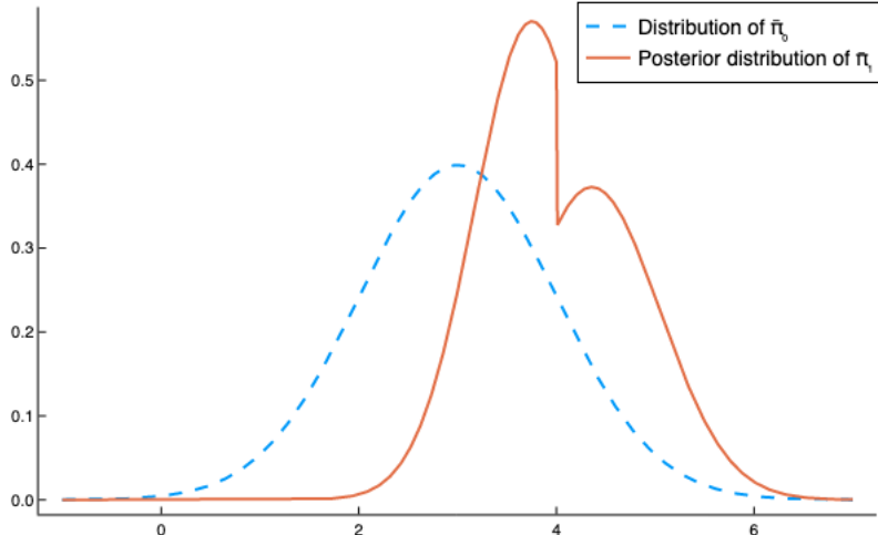
Figure 1: Prior distribution of \bar{\pi}_0 and posterior distribution of \bar{\pi}_1 .
