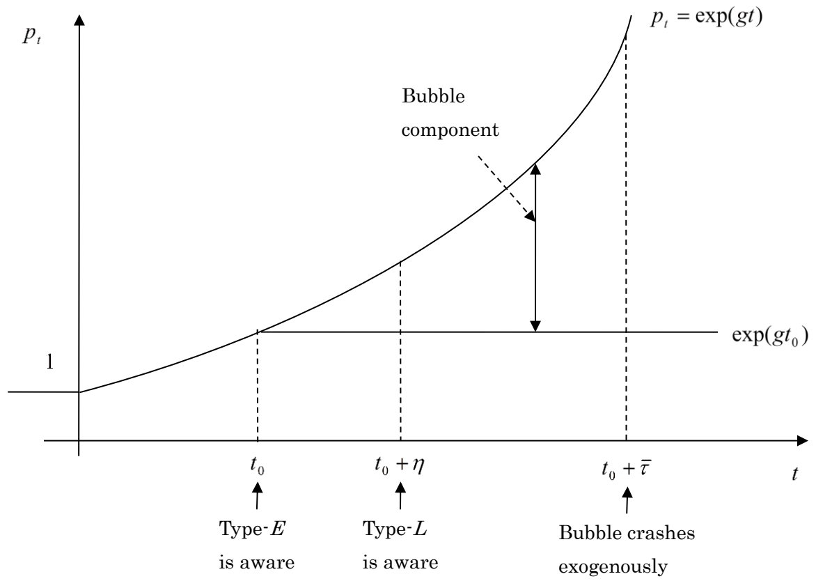
Figure 1: Riding-bubble Model
