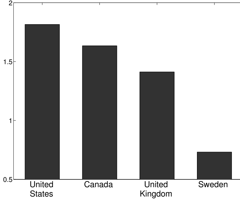
Figure 10: Conditional Averages of Inflation Away From the ELB †
