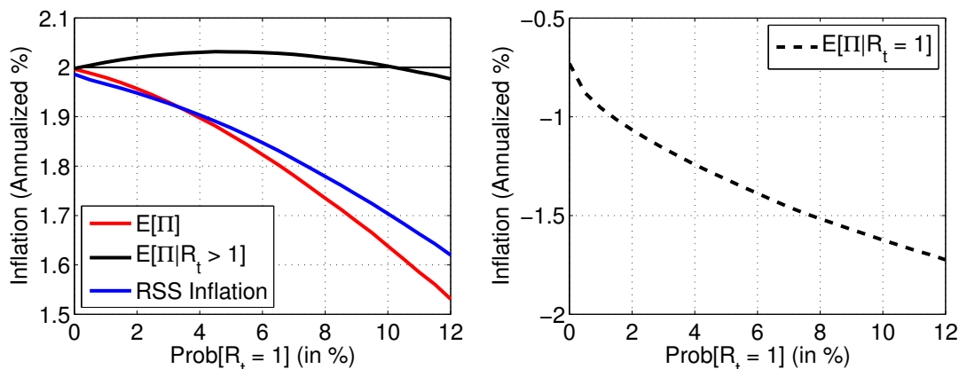
Figure 3: Conditional and Unconditional Averages of Inflation in the Stylized Model
