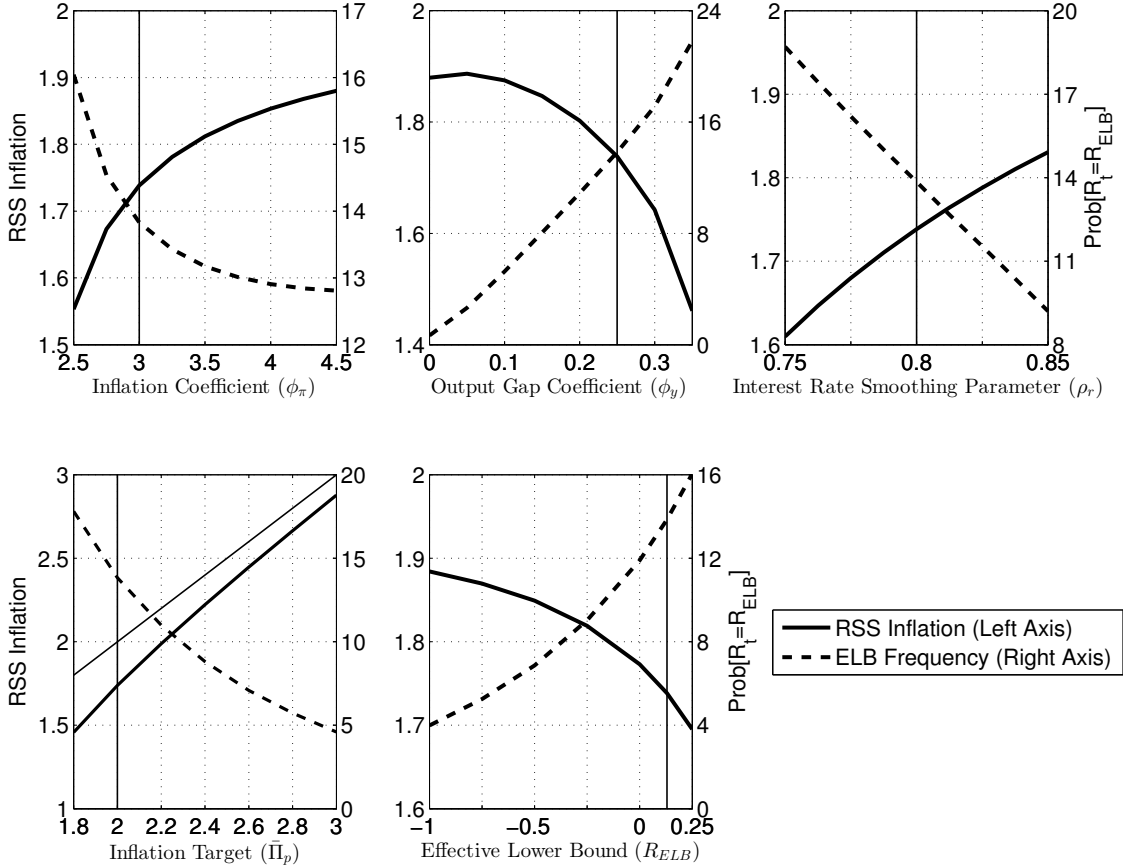
Figure 9: Alternative Policy Parameters †
