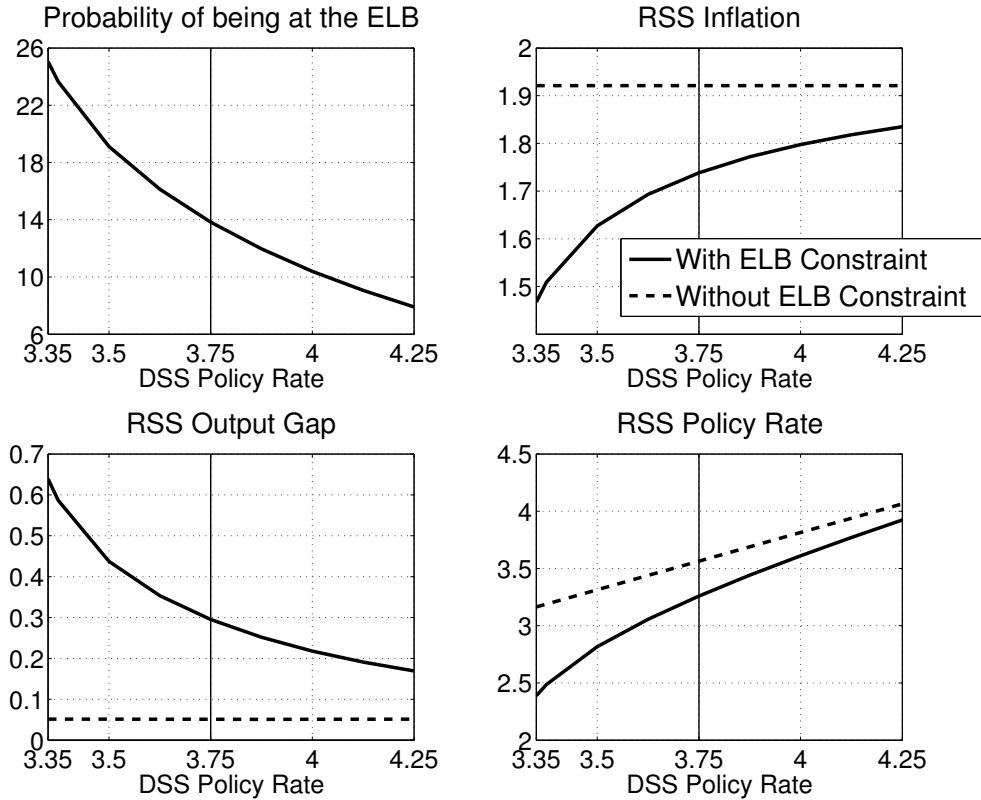
Figure 8: Long-Run Interest Rates and the Risky Steady State †
