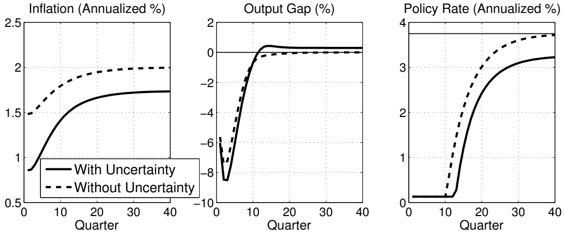
Figure 7: The Effect of the ELB Risk
